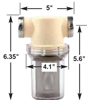
1-1/4" Strainer 18016
