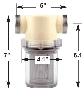
1" Strainer 18005
