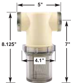
1-1/2" Strainer 18029
